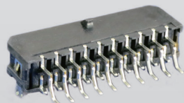
P/N:4312-SXX2RC-RN Dwg:4312-2RM
