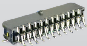
P/N:4312-SXX2RF-RN Dwg:4312-2RM
